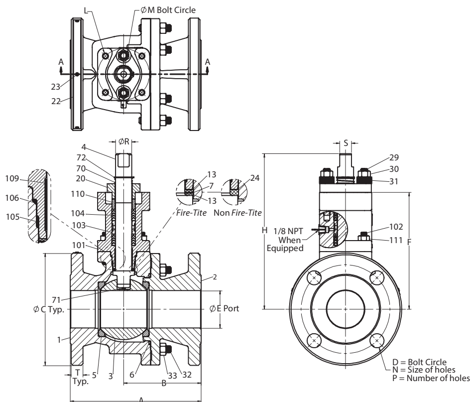
Series 9150 ASME Class 150 Approximate Dimensions - inches Valve Size inches A B C D E F H L M N P R S T ISO Pattern Weight lb 2 7.00 4.14 6.00 4.75 2.00 6.24 8.31 M8 2.76 0.75 4 0.86 0.62 0.62 F07 39 3 8.00 4.26 7.50 6.00 3.00 7.06 9.11 M8 2.76 0.75 4 0.86 0.62 0.75 F07 59 4 9.00 4.50 9.00 7.50 4.00 9.45 12.18 M10 4.02 0.75 8 1.11 0.81 0.94 F10 105 6 15.50 8.25 11.00 9.50 6.00 11.39 14.49 M12 4.92 0.88 8 1.61 1.12 1.00 F12 276
