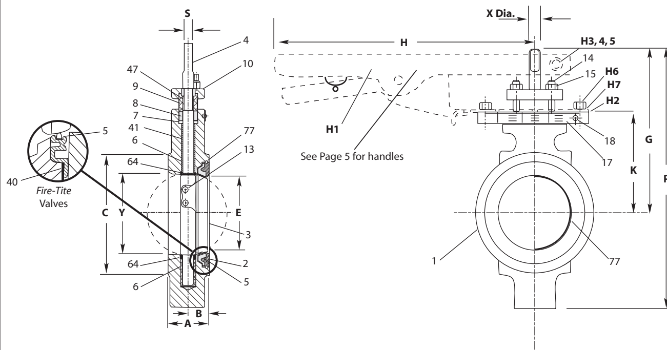
2-1/2" – 12" (DN 65 – 300) Type 815W (Model C) Valves ANSI Class 150, Series 815 Wafer Design
