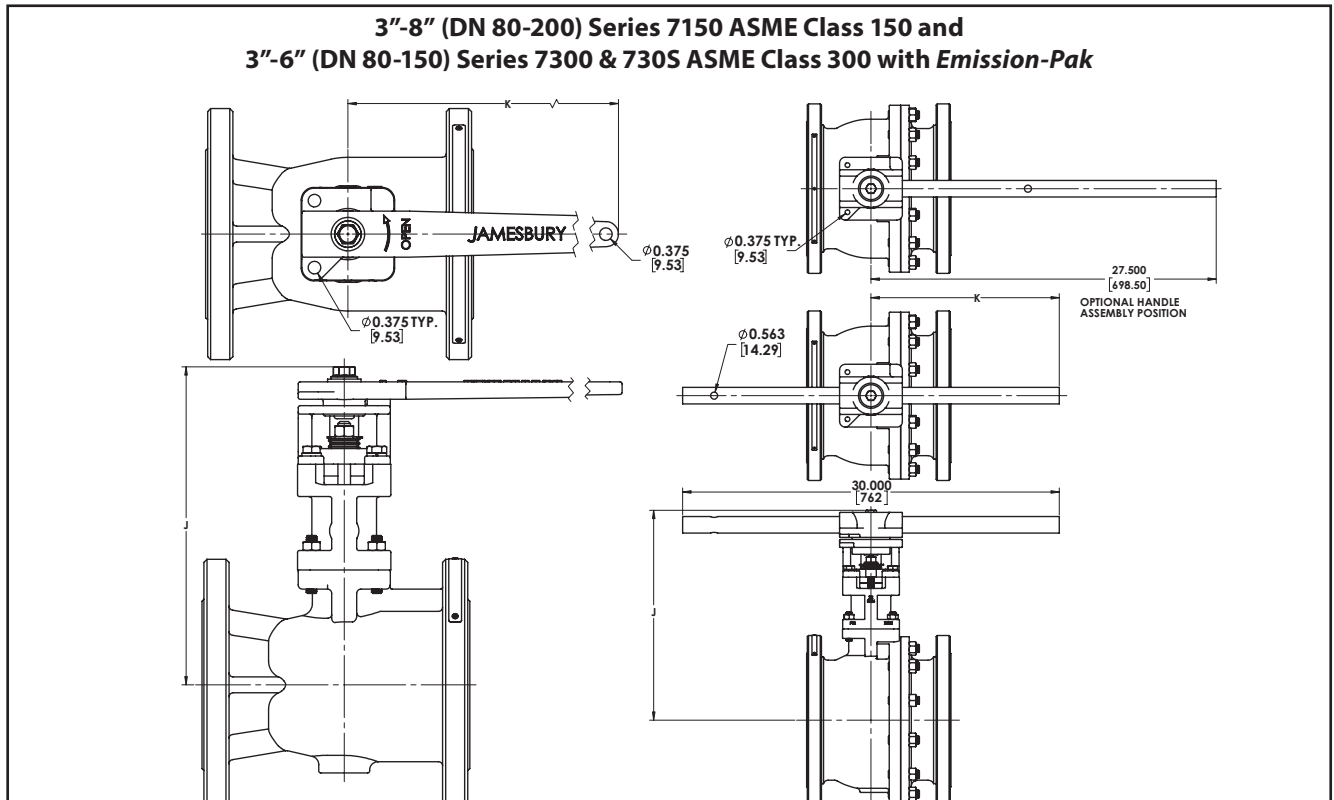
Series 7150 ASME Class 150 Approximate Dimensions - inches
